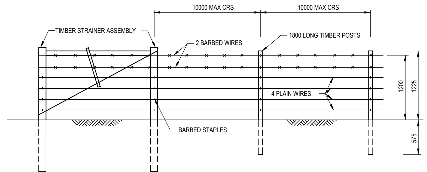
TYPICAL PLAIN OR BARBED WIRE FENCE TIMBER STRAINERS AND POSTS
