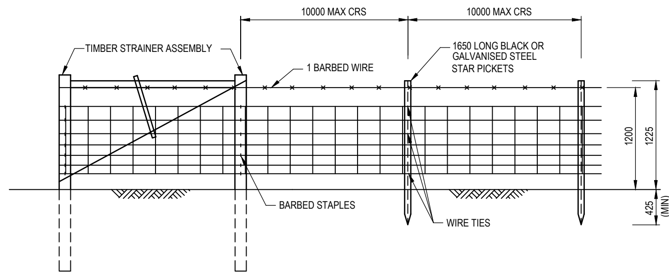
TYPICAL PREFABRICATED FENCEWIRE (MESH) FENCE TIMBER STRAINERS AND STEEL POSTS
