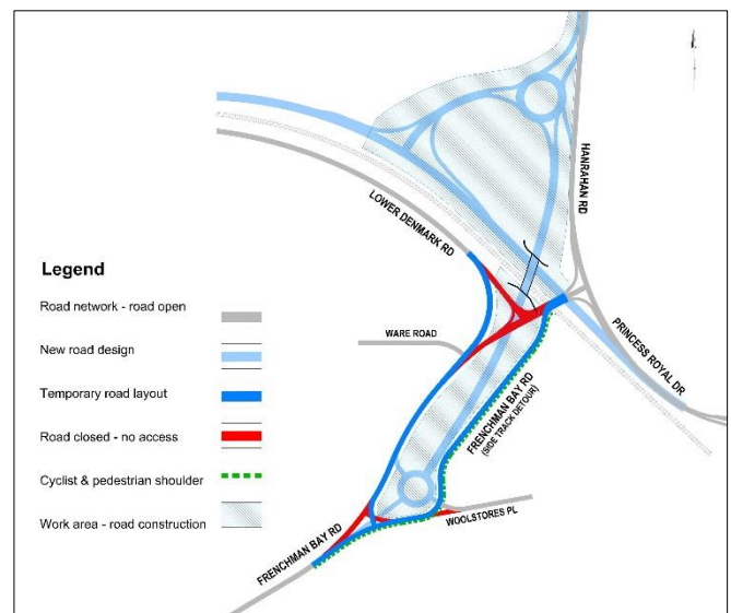
Figure 1: Temporary road layout: Hanrahan Road / Frenchman Bay Road
