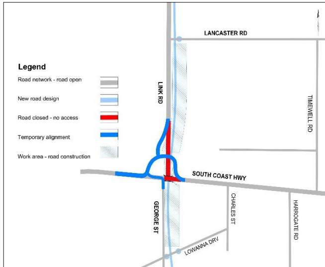
Figure 2: Temporary road layout: South Coast Highway
