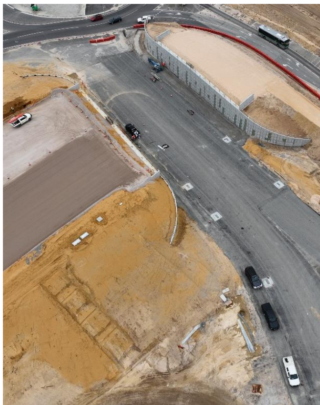
Image (above): Altone Road bridge construction ahead of beam installation.
