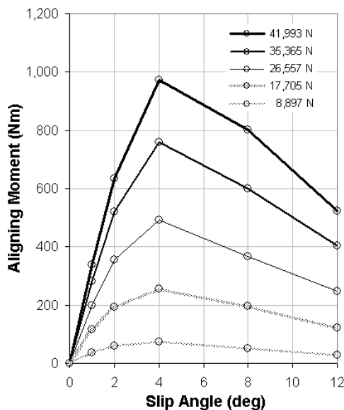
Figure 23. Aligning moment characteristics of an 11R22.5 size truck tyre showing the influence of tyre vertical load.
