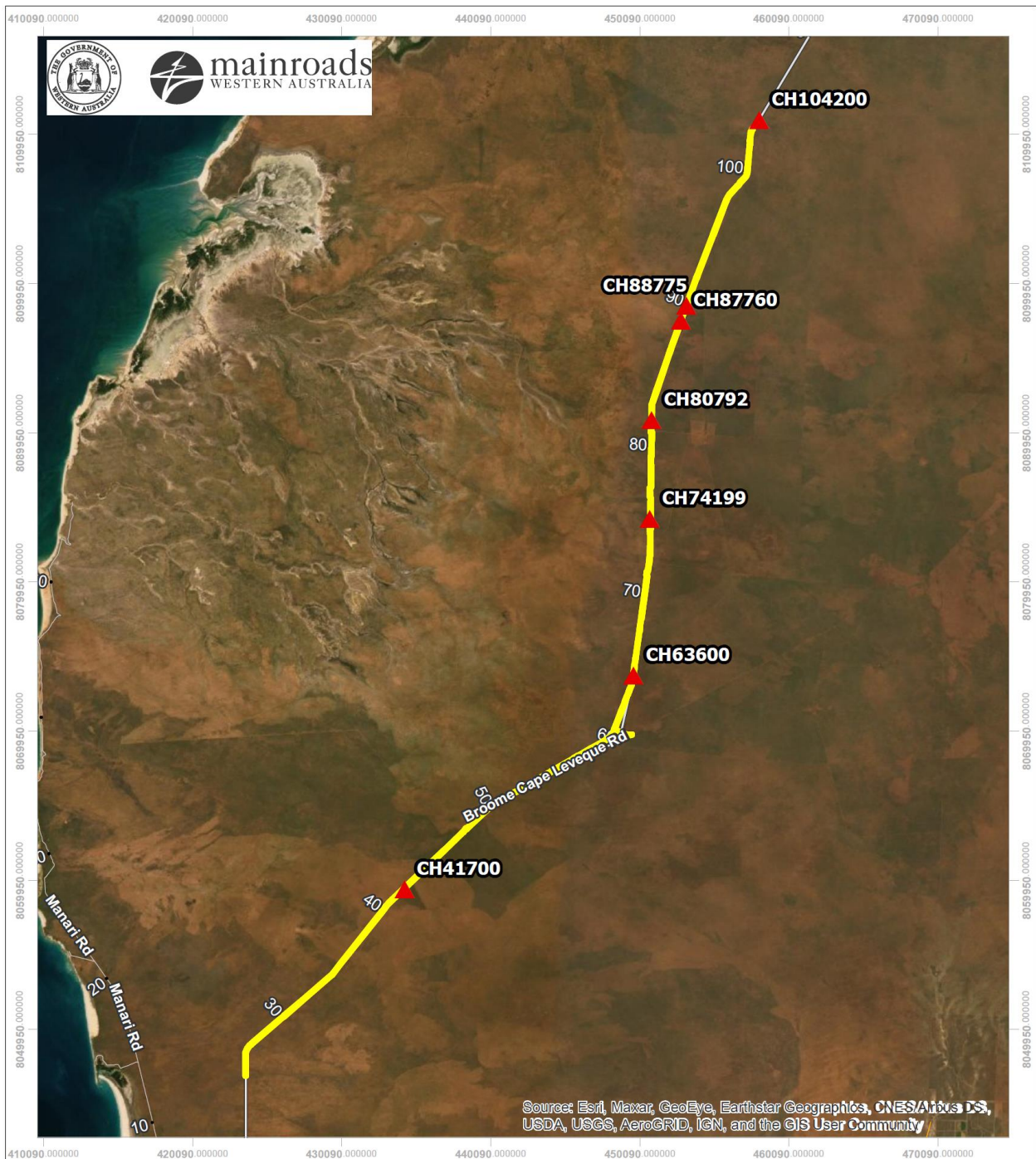
Figure 1 Broome-Cape Leveque Road Fauna Underpasses
