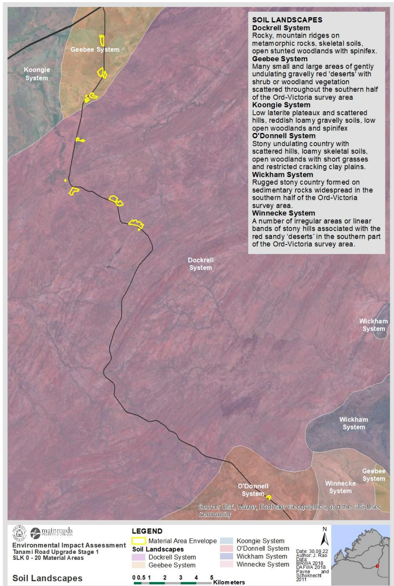
Figure 5. Soil Landscapes
