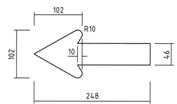
ARROW DETAIL
