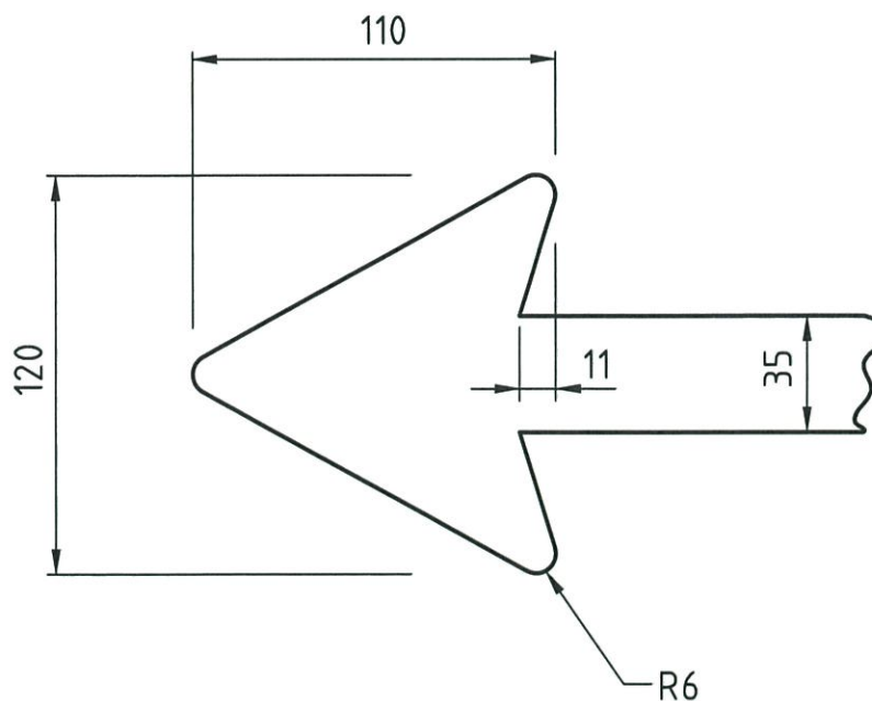
ARROW DETAIL SCALE 1:2.5
