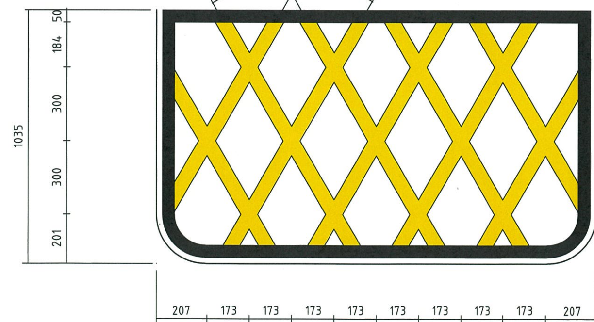
PART B YELLOW CROSS HATCHING LAYOUT DETAILS
