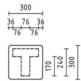
SYMBOL DETAIL
