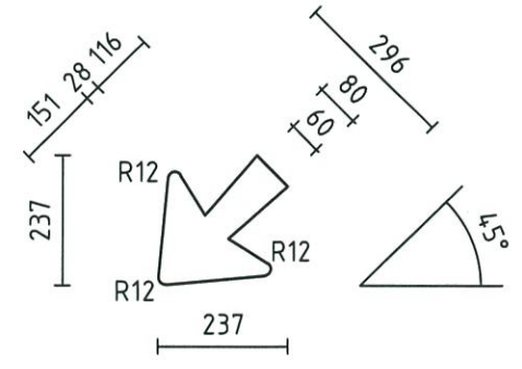
ARROW DETAIL
