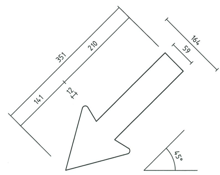
ARROW DETAIL SCALE 1:5
