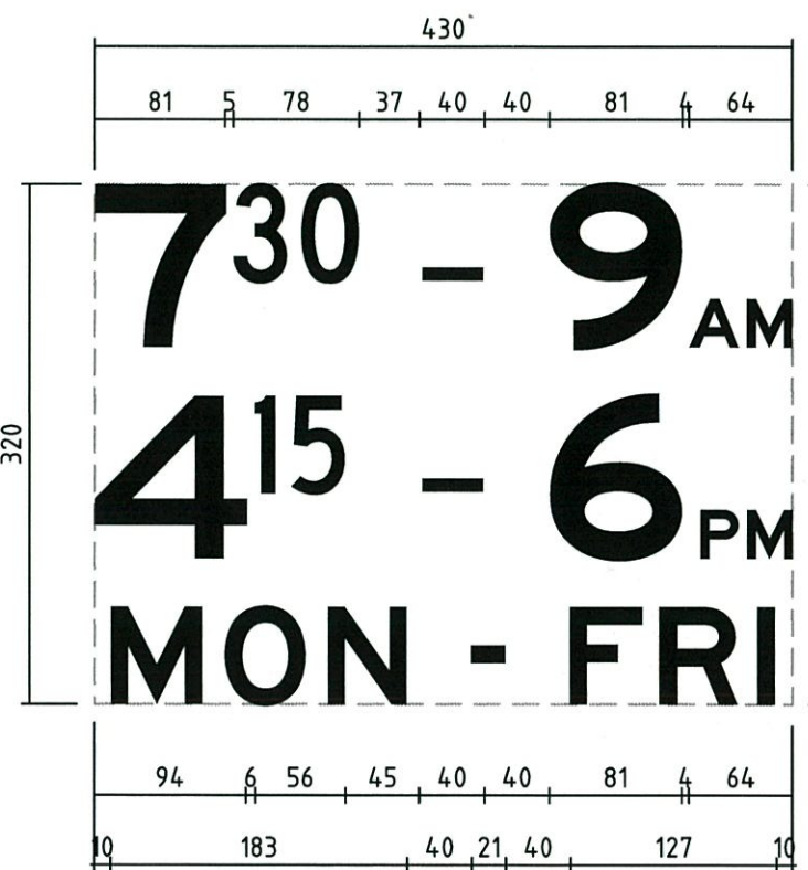
DETAIL (A) 1:5
