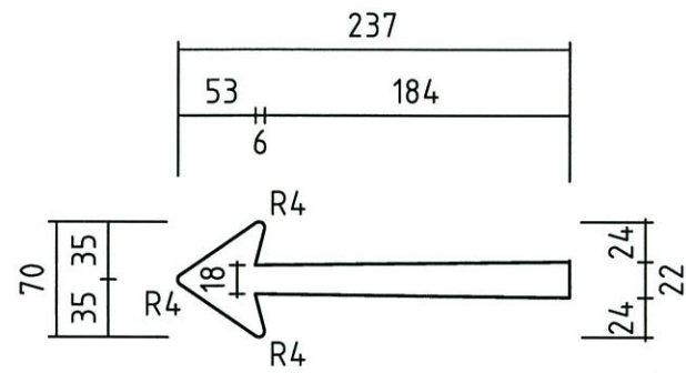
ARROW DETAIL
