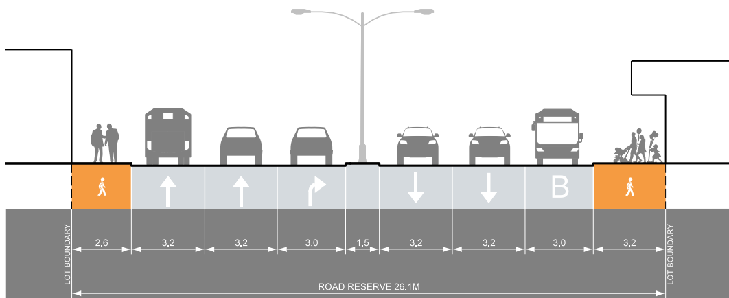
Proposed Cross-Section
