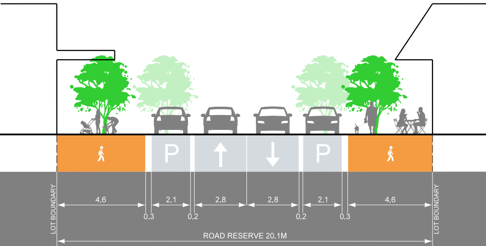
Proposed Cross-Section
