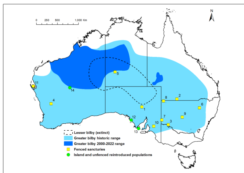
Fig. 1 Current and former Greater and Lesser Bilby distribution. Reintroduced or introduced populations of the Greater Bilby: 1 Arid Recovery, 2 Currawinya, 3 Mallee Cliffs, 4 Mt Gibson, 5 Newhaven, 6 Pilliga, 7 Scotia, 8 Sturt, 9 Yathong, 10 Yookamurra, 11 Peron, 12 Venus Bay, 13 Thistle Is, 14 Matuwa.
