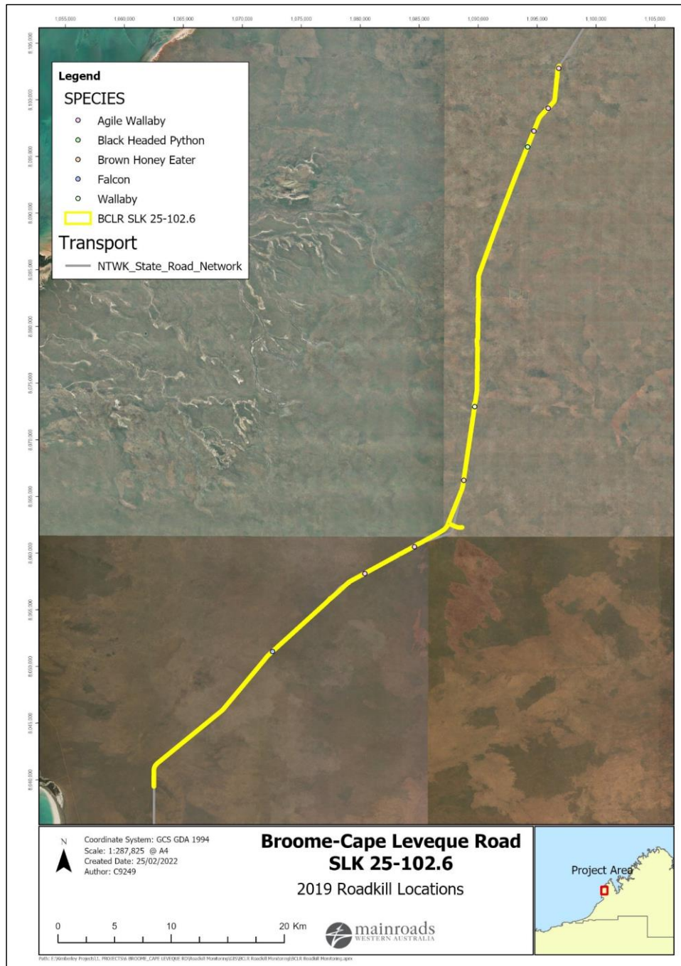
Figure 6: 2019 Roadkill Locations
