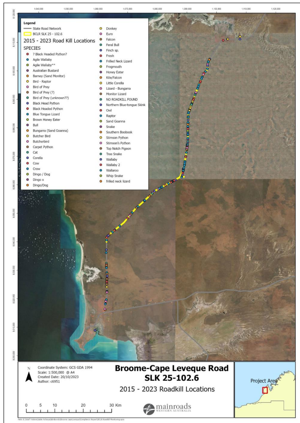
Figure 11: 2015 – 2023 Roadkill Locations
