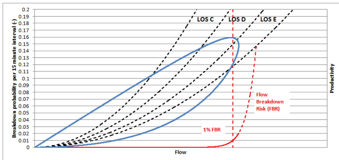
Figure 1-3: Breakdown probability and productivity plotted against traffic flow
