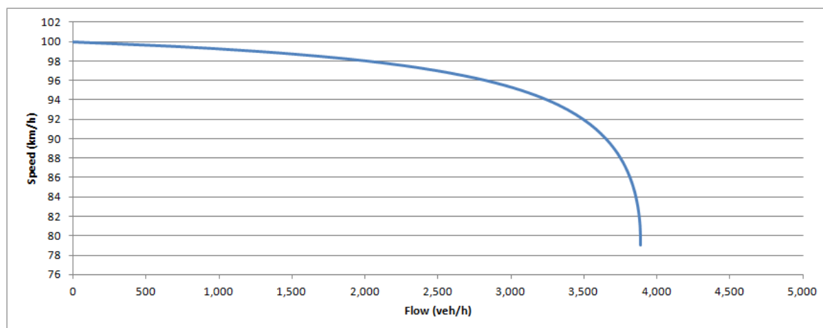
Figure 2-14: Average vehicle speed for 2 lane cross-sections (100 km/h speed limit)
