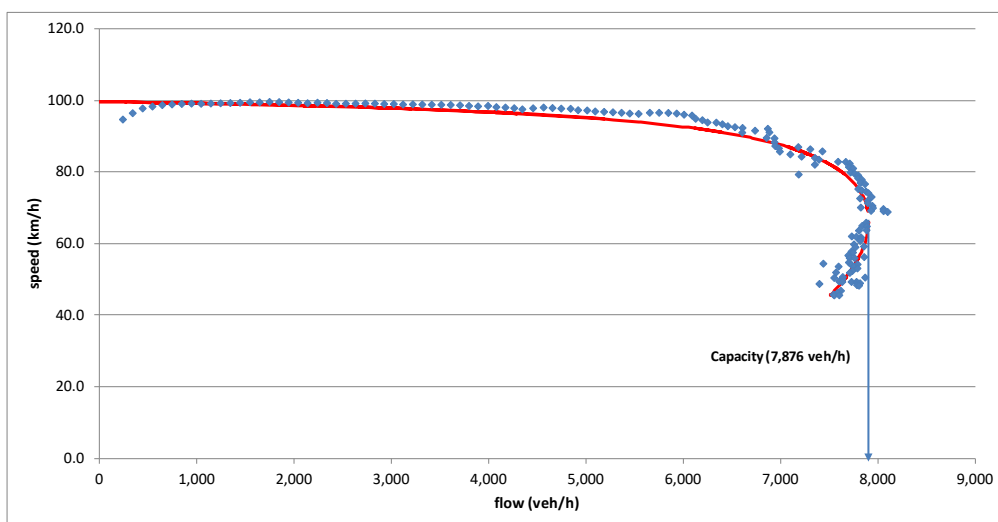
Figure 3-4: Speed-flow relation for cross-section 14587IB (Monash Freeway - Jacksons to Wellington Road, inbound, 4 lanes) - measured values (1 hour rolling averages aggregated for density classes) and van Aerde curve approximation (elimination of downstream bottleneck influence)
