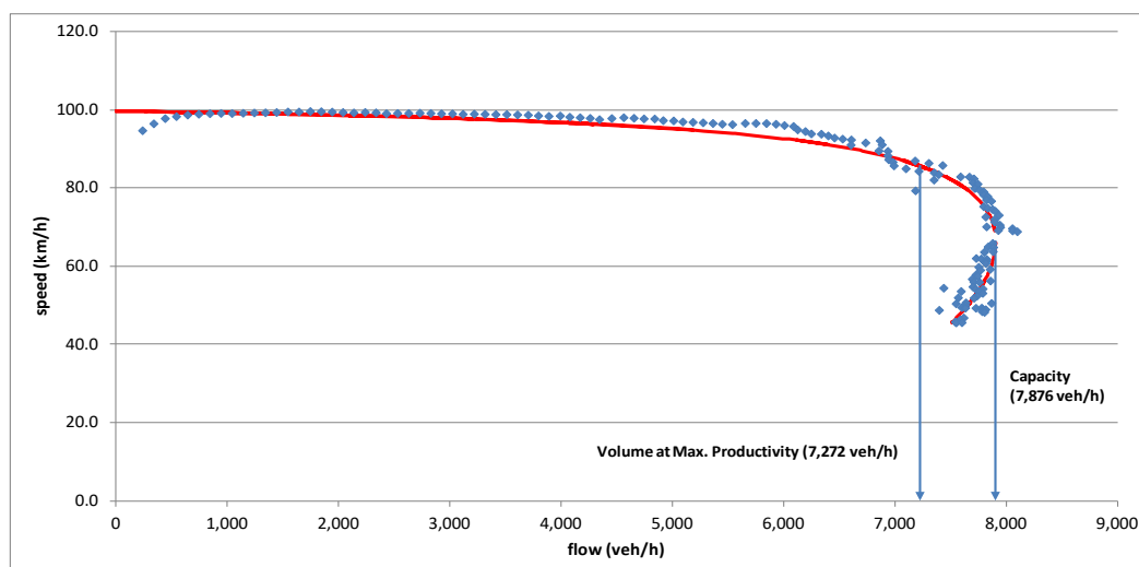
Figure 3-6: ‘Capacity’ and volume at maximum productivity for cross-section 14587IB (1 hour rolling averages aggregated for density classes)
