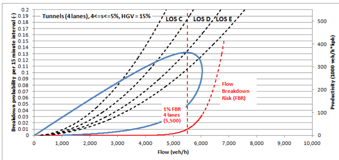
Figure 2-8: Breakdown probability and productivity plotted against flow rate (4 lane tunnels)
