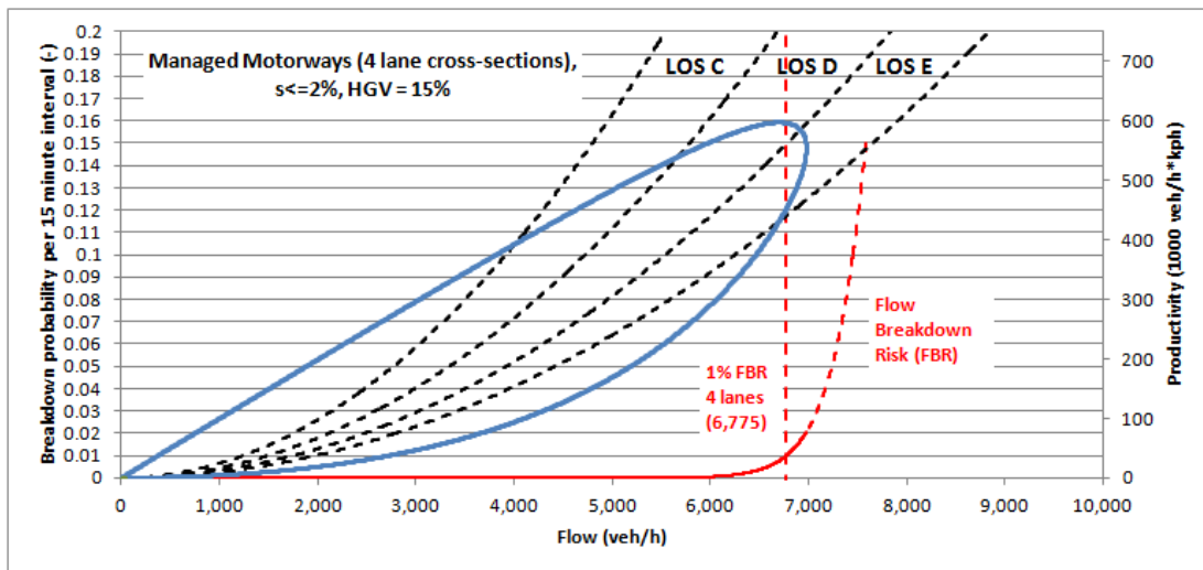
Figure 2-3: Breakdown probability and productivity plotted against flow rate (4 lane cross-sections)
