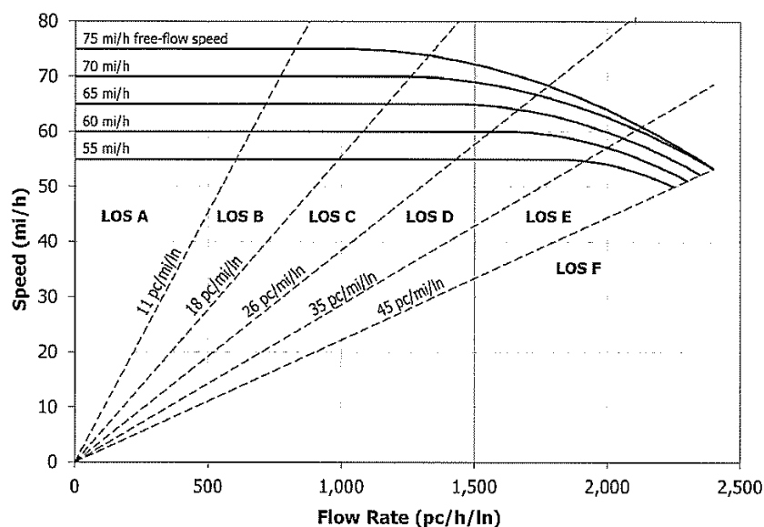
Figure 1-1: General relationship between speed and flow rate (Source: HCM 2016)
