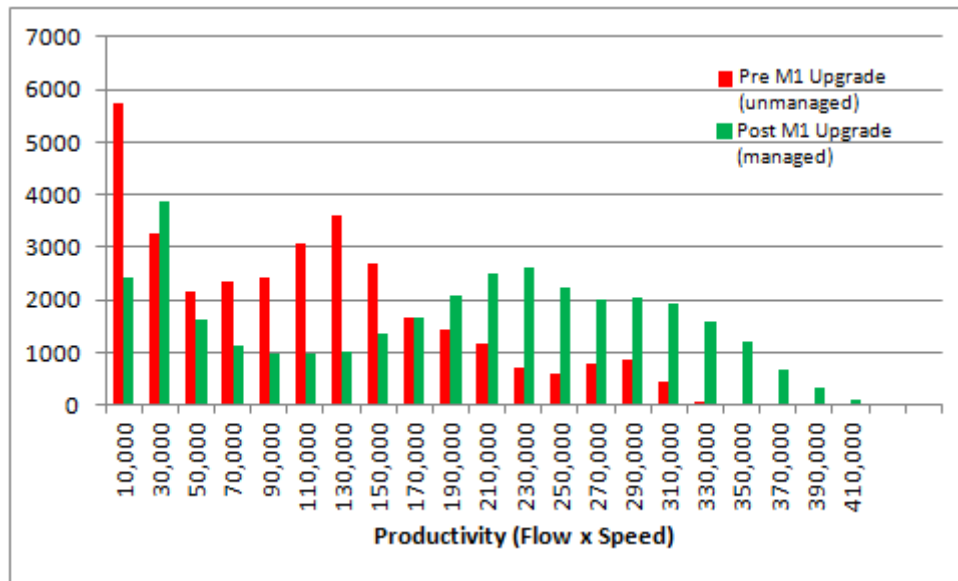
Figure 3-9: Example for a Productivity Frequency Plot (14316 OB and 14456 OB, 15 min intervals)
