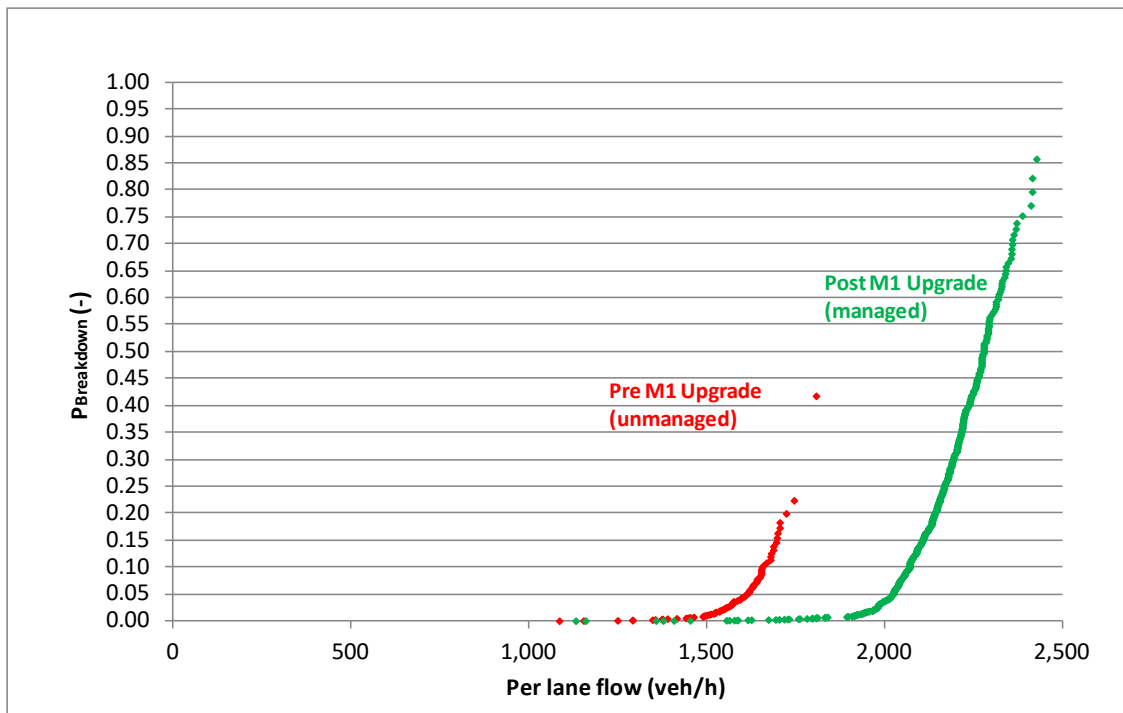
Figure 3-8: Flow breakdown probability on Hallam Bypass – before and after M1 Upgrade (14316 OB and 14456 OB, 15 min intervals)
