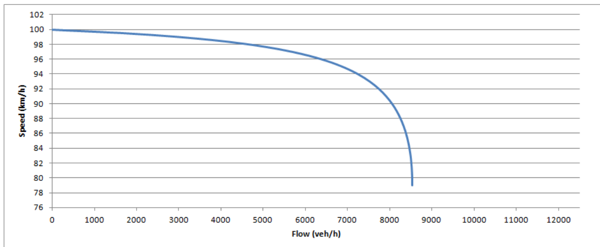
Figure 2-17: Average vehicle speed for 5 lane cross-sections (100 km/h speed limit)
