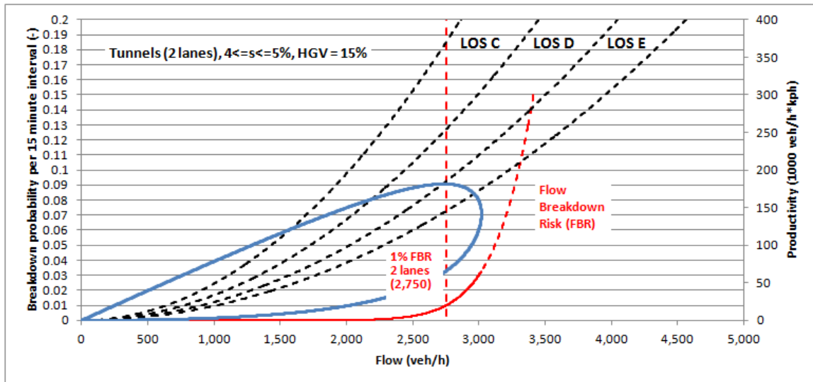
Figure 2-6: Breakdown probability and productivity plotted against flow rate (2 lane tunnels)
