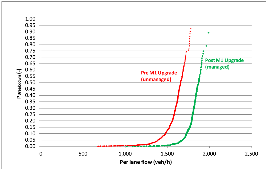
Figure 3-7: Flow breakdown probability at Warrigal Road - before and after M1 Upgrade (7839 OB and 14547 OB, 15 min intervals)
