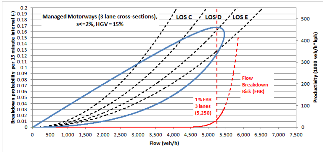
Figure 2-2: Breakdown probability and productivity plotted against flow rate (3 lane cross-sections)
