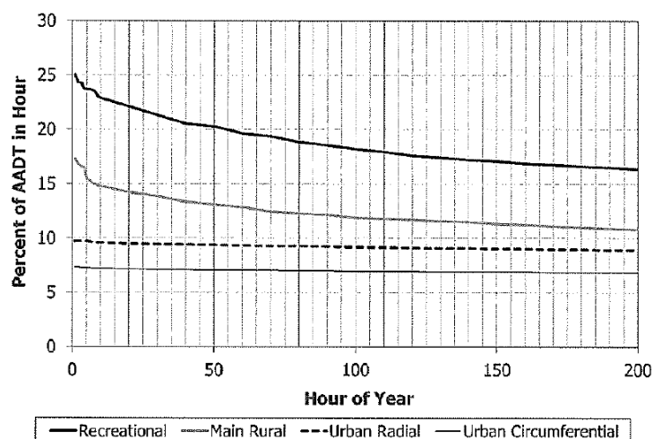
Figure 2-19: Typical relationships between hourly volumes and AADT (Source: HCM, 2016)
