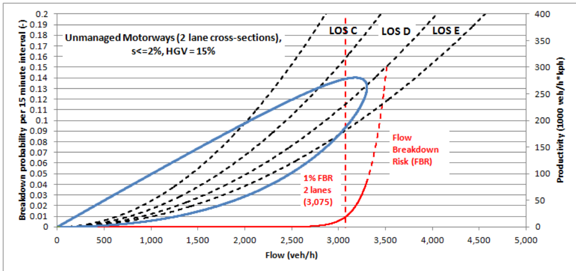
Figure 2-10: Breakdown probability and productivity plotted against flow rate (2 lane cross-sections)
