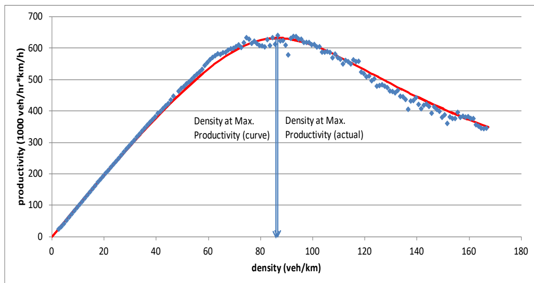
Figure 3-5: Carriageway productivity-density relation for cross-section 145871B (1 hour rolling averages aggregated for density classes)
