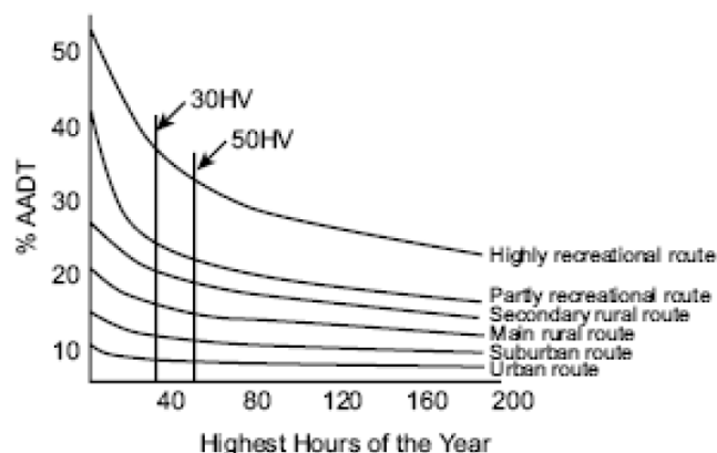
Figure 2-18: Typical relationships between hourly volumes and AADT (Source: Austroads, 2013)
