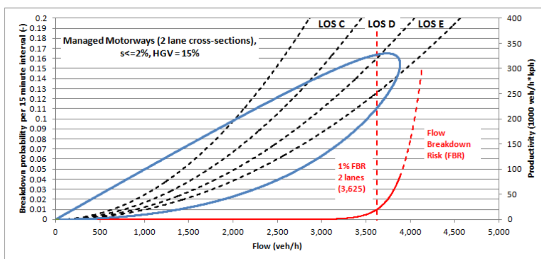
Figure 2-1: Breakdown probability and productivity plotted against flow rate (2 lane cross-sections)
