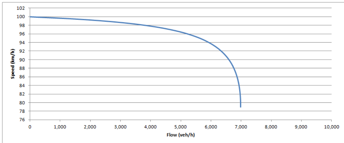
Figure 2-16: Average vehicle speed for 4 lane cross-sections (100 km/h speed limit)
