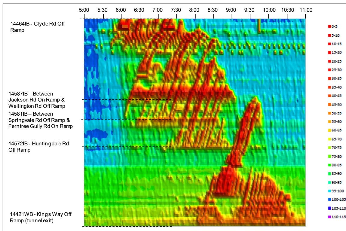
Figure 3-2: 'Heat Plot' from the Monash Freeway (inbound speed profile)
