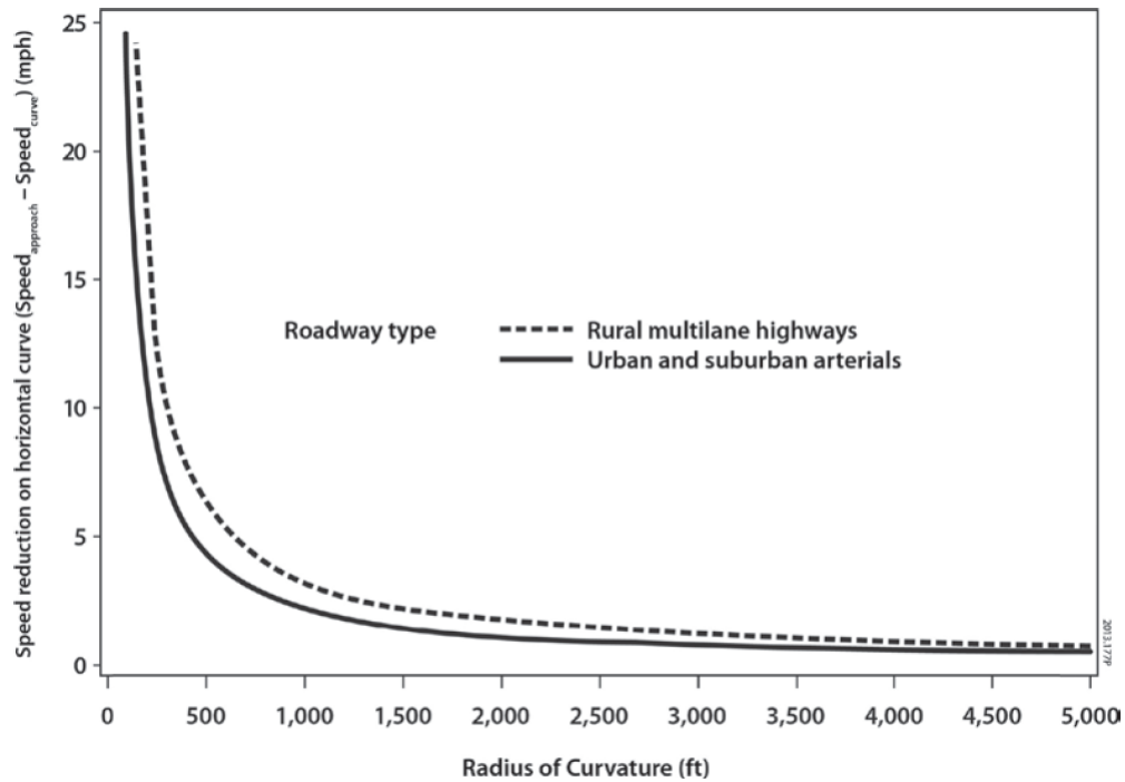
Figure 3-11: Speed reduction on curves (Harwood et al., 2014)
