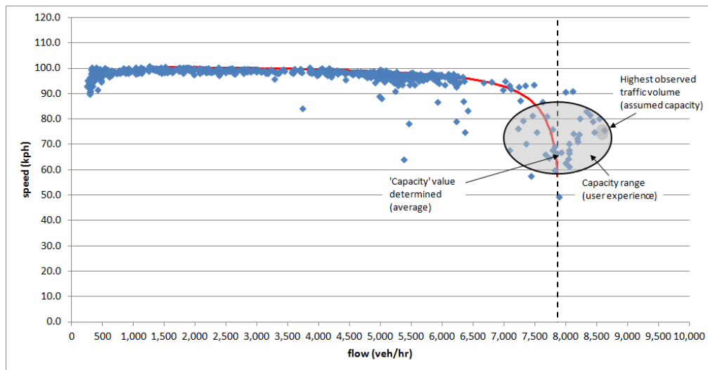
Figure 1-2: 'Highest observed traffic volume' versus 'Capacity value determined' (actual 1 hour speed and flow data measured over 1 month; Monash Freeway 4 lane cross-section 14587 IB, Jacksons Rd to Wellington Rd)
