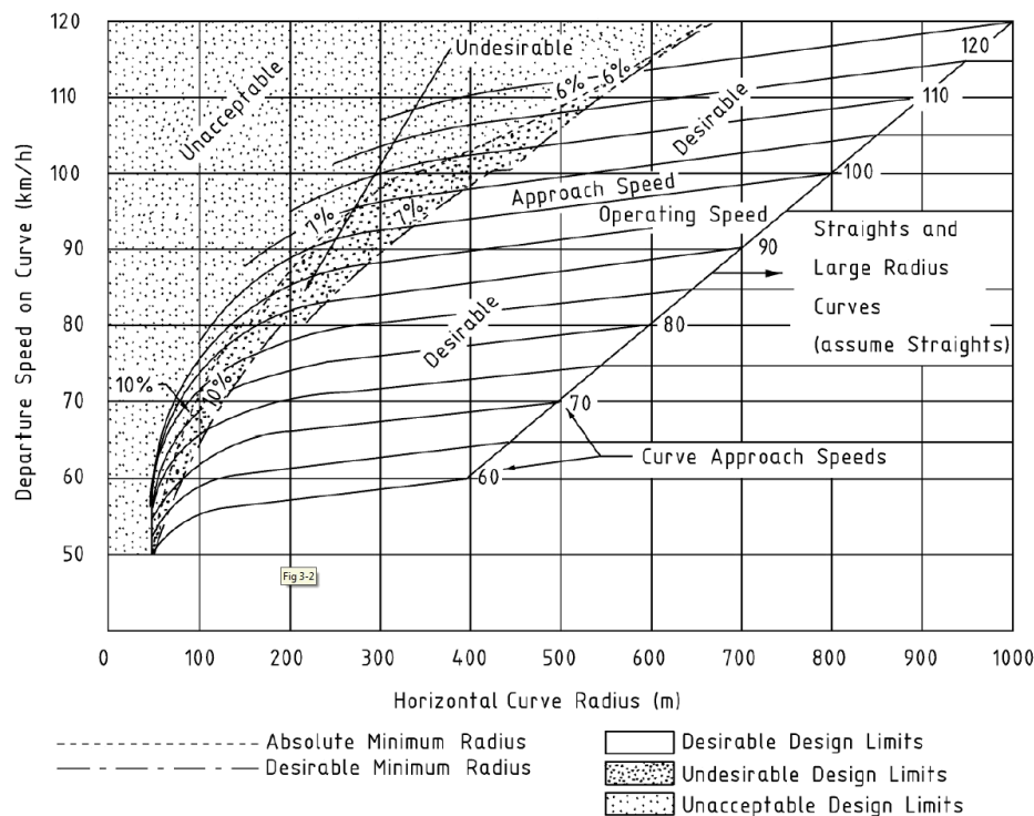
Figure 3-10: Car deceleration on curves (Austroads, 2016)
