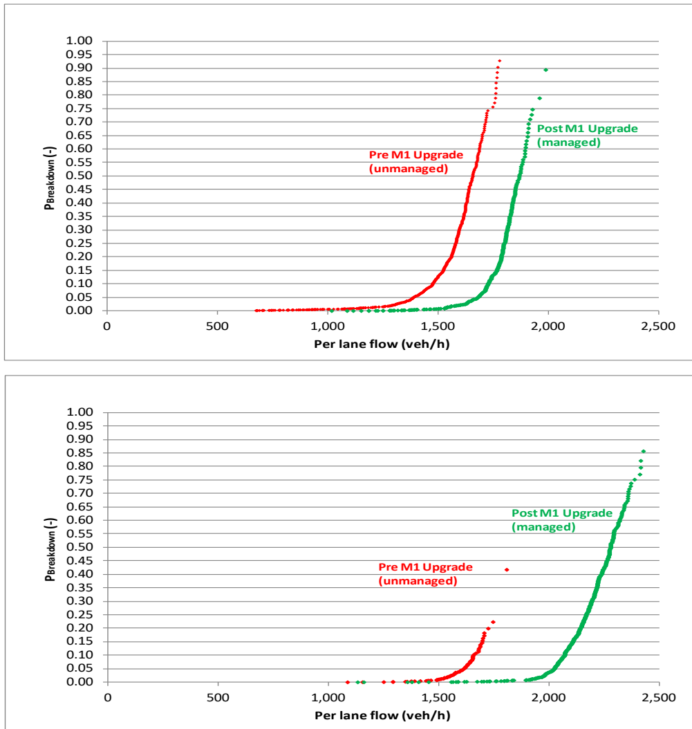
Figure 2-9: Flow breakdown probability over 15 minutes for managed and unmanaged motorways (Warrigal Road (3 lanes, top) and Hallam Bypass (2 lanes, bottom), outbound direction)
