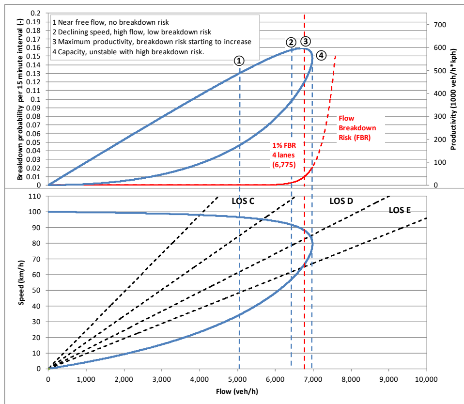
Figure 1-5: Breakdown probability, productivity and speed plotted against flow rate (4 lane cross-sections)
