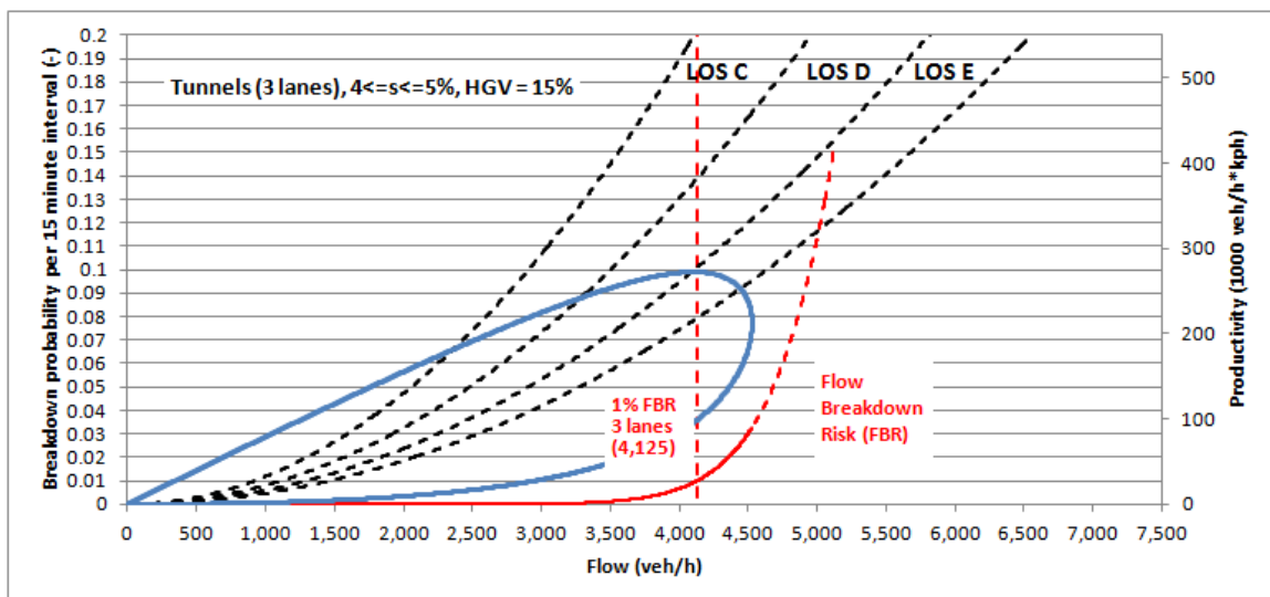
Figure 2-7: Breakdown probability and productivity plotted against flow rate (3 lane tunnels)
