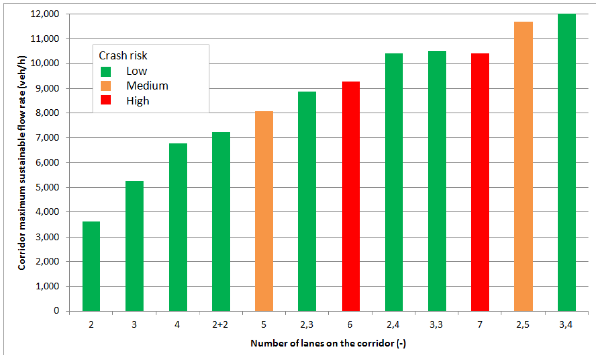
Figure 2-5: Corridor Maximum Sustainable Flow Rates under various lane configurations 1
