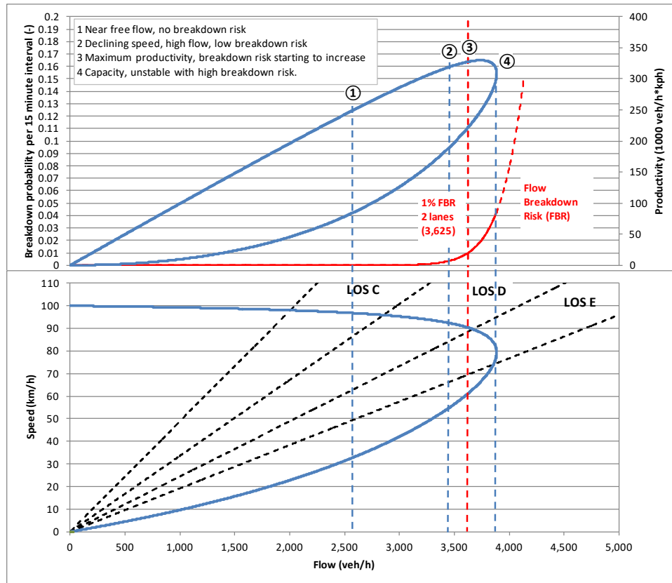
Figure 1-4: Breakdown probability, productivity and speed plotted against flow rate (2 lane cross-sections)
