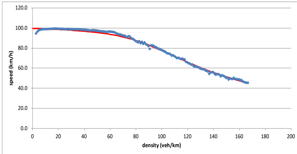
Figure 3-3: Speed-density relation for cross-section 14587IB (Monash Freeway - Jacksons to Wellington Road, inbound, 4 lanes) - measured values (1 hour rolling averages aggregated for density classes) and van Aerde curve approximation (elimination of downstream bottleneck influence – hence no very high densities)
