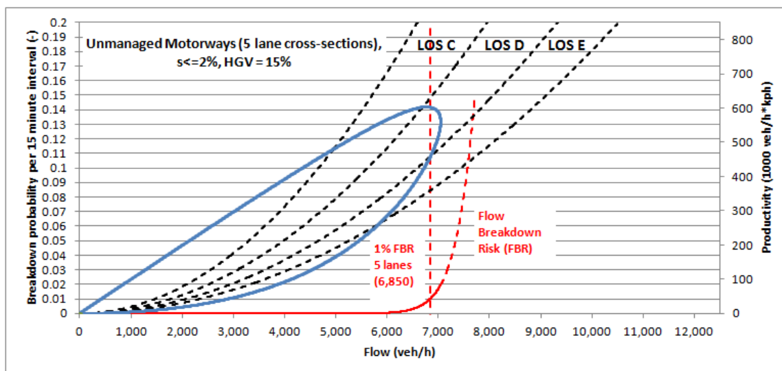
Figure 2-13: Breakdown probability and productivity plotted against flow rate (5 lane cross-sections)
