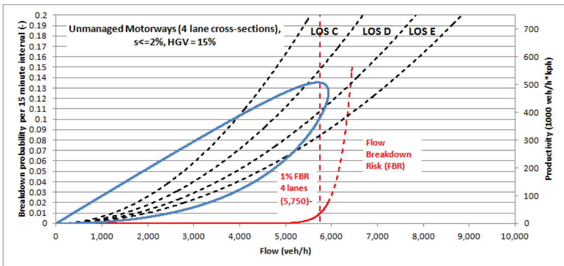
Figure 2-12: Breakdown probability and productivity plotted against flow rate (4 lane cross-sections)
