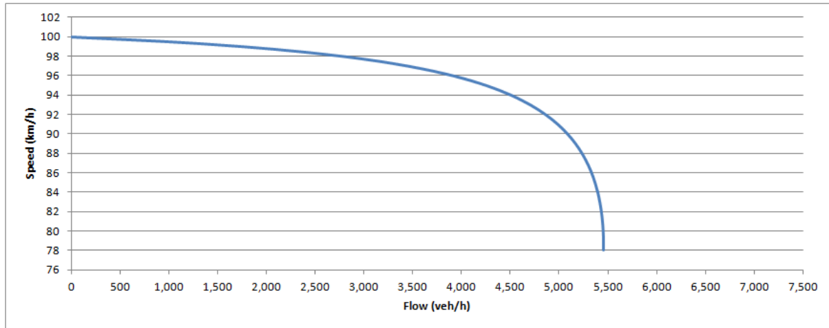
Figure 2-15: Average vehicle speed for 3 lane cross-sections (100 km/h speed limit)
