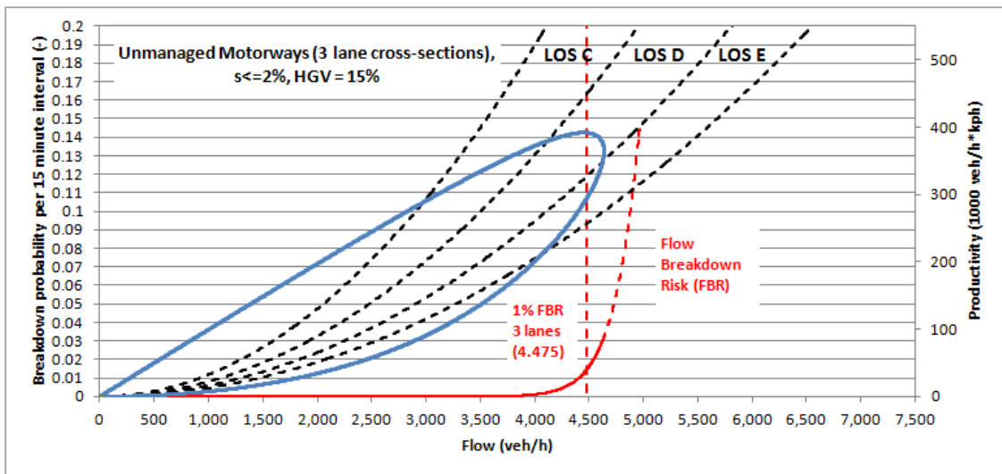
Figure 2-11: Breakdown probability and productivity plotted against flow rate (3 lane cross-sections)
