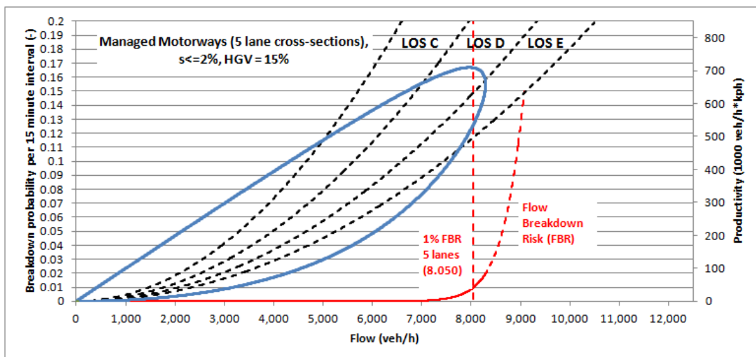
Figure 2-4: Breakdown probability and productivity plotted against flow rate (5 lane cross-sections)
