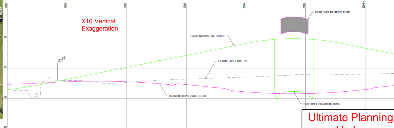
RAYMOND ROAD PROFILE SCALE 1:1000 HOR, 1:100 VERT
