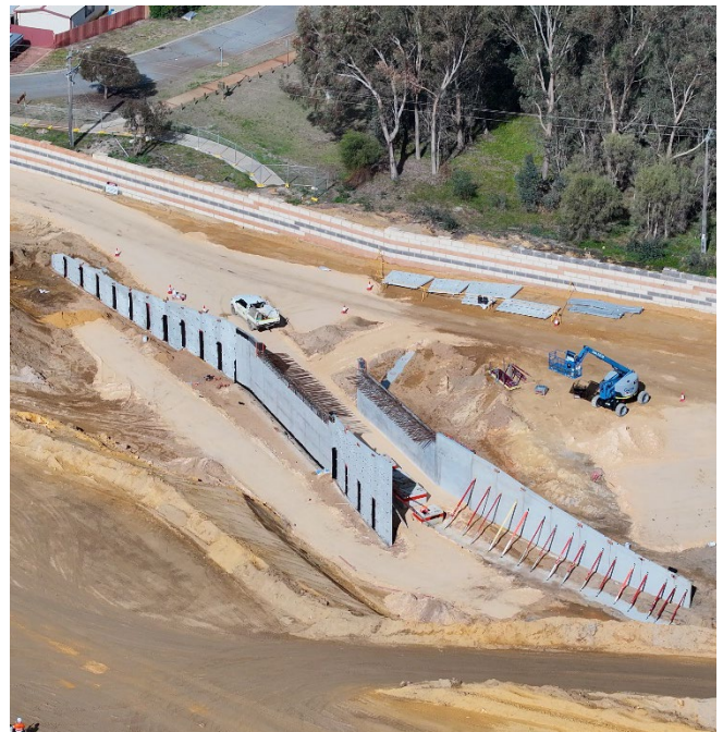
Image: MSE panel installation – shared path underpass at Reid Highway / Altone Road.
