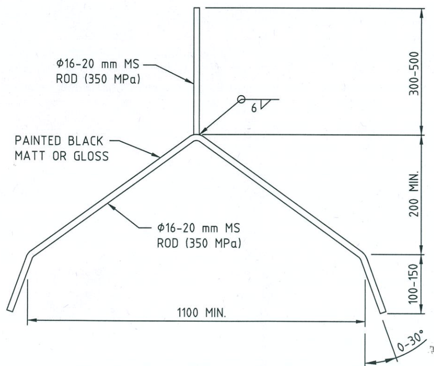
GROUND SUPPORT STANDS
