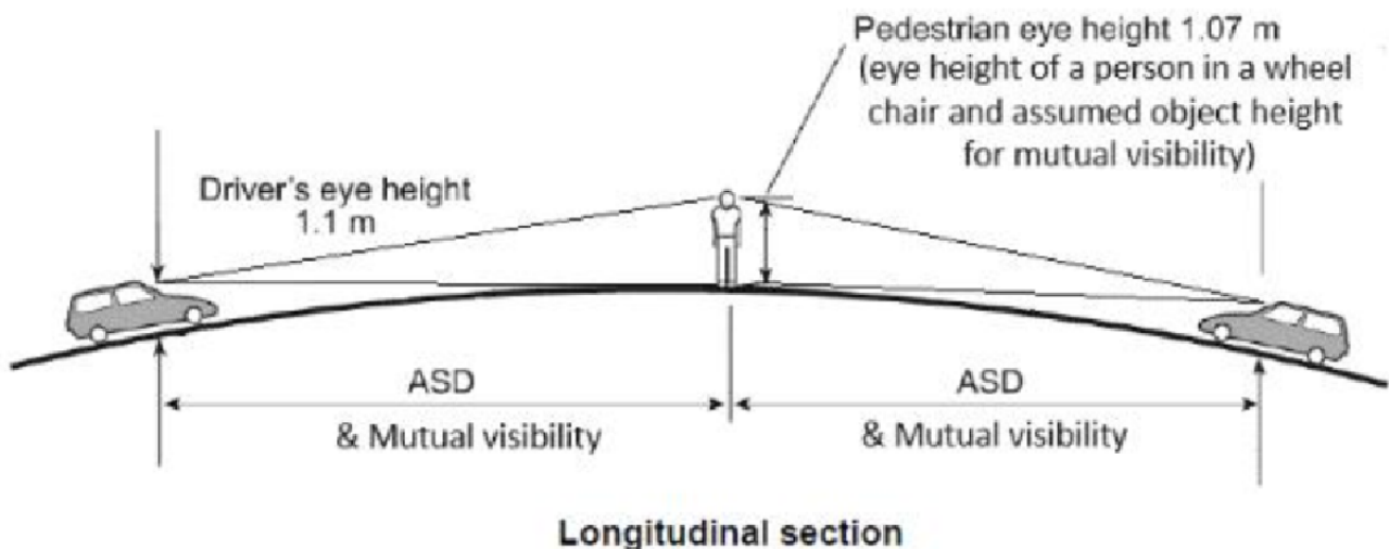
Figure 3.7(a): Sight distance required at marked (priority) pedestrian crossings
