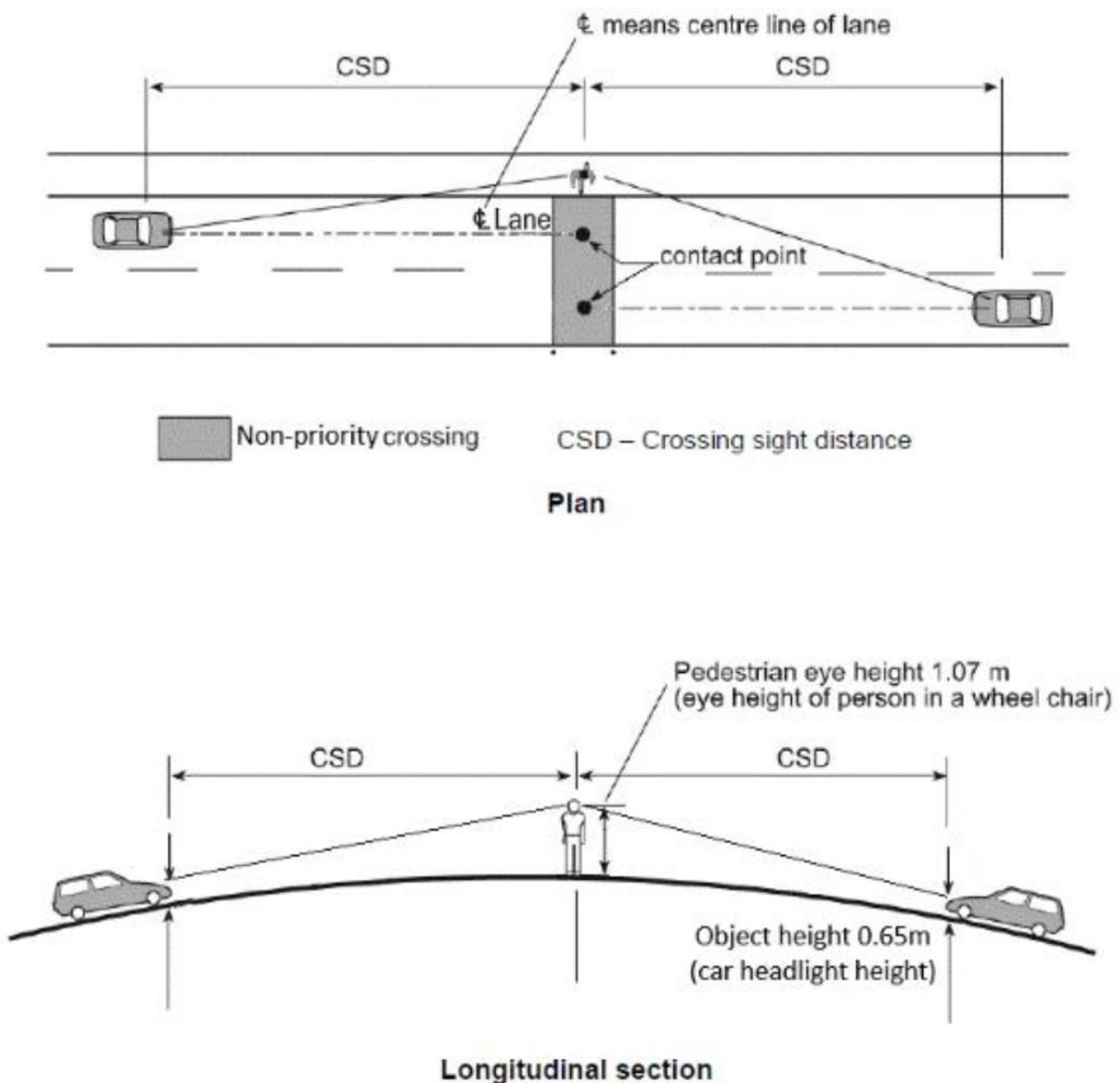
Figure 3.7(b): Sight distance required at unmarked (non-priority) pedestrian crossings
