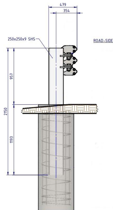
Typical Cross Section thru Abutment Post
