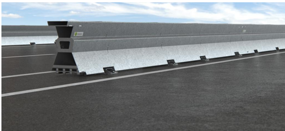
Photograph of Installation (4# anchor shoes shown – i.e. end anchor)
