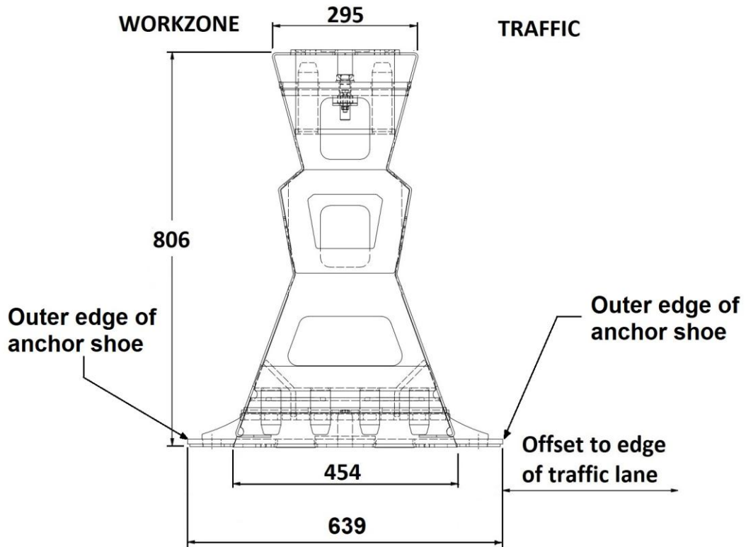
Cross section (anchor shoes shown)
