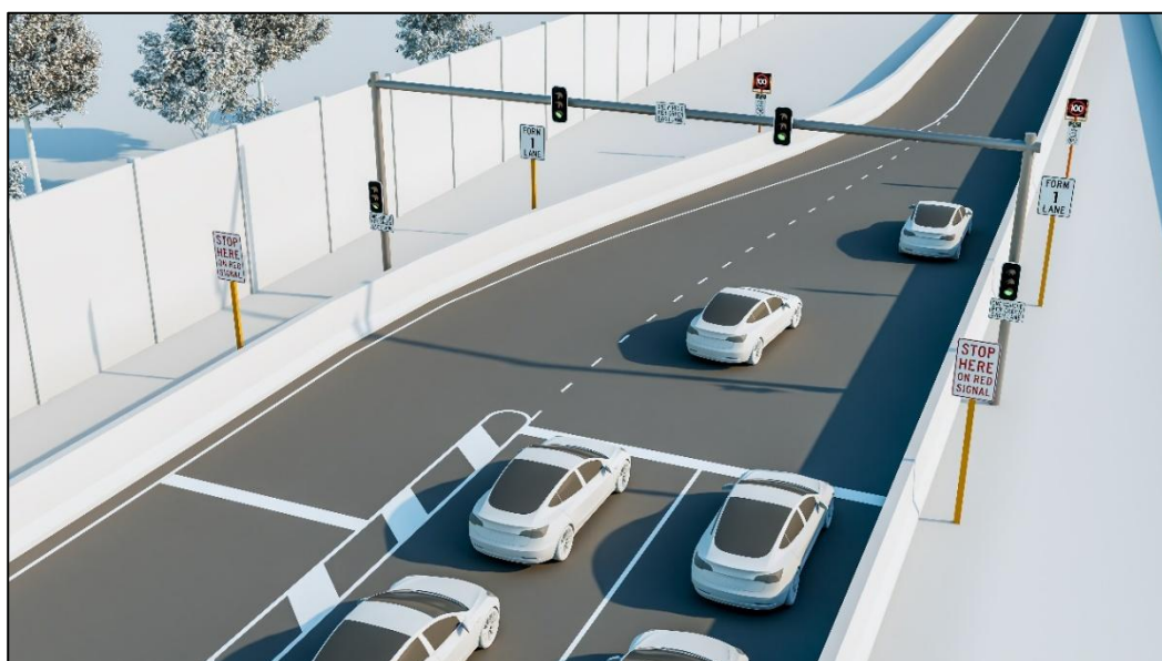
Figure 2-1: Coordinated ramp signals on the entry ramps of the freeway
