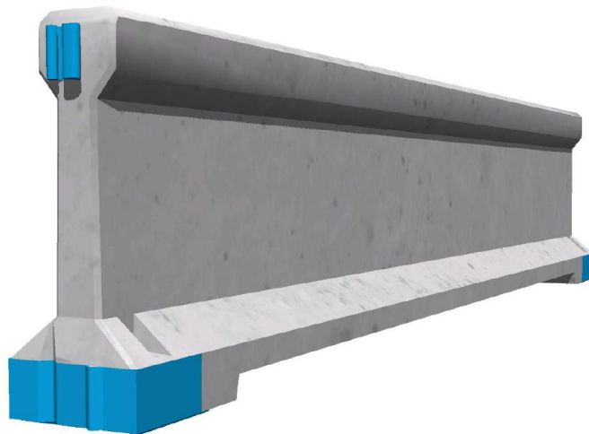
Image of 4 m long REBLOC 80SAH_4 unit
