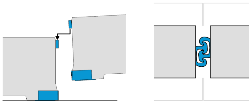
Images of REBLOC 80SAH_4 Joints
